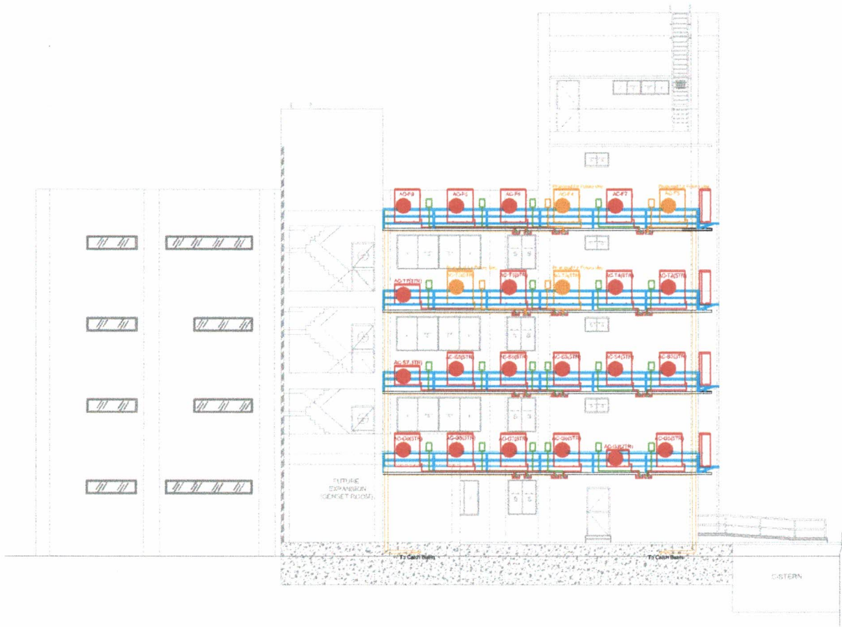
2 REAR ELEVATION AR-5 SCALE: 0 0.5 1.0 2.0 3.0 5.0 1:100 MTS
