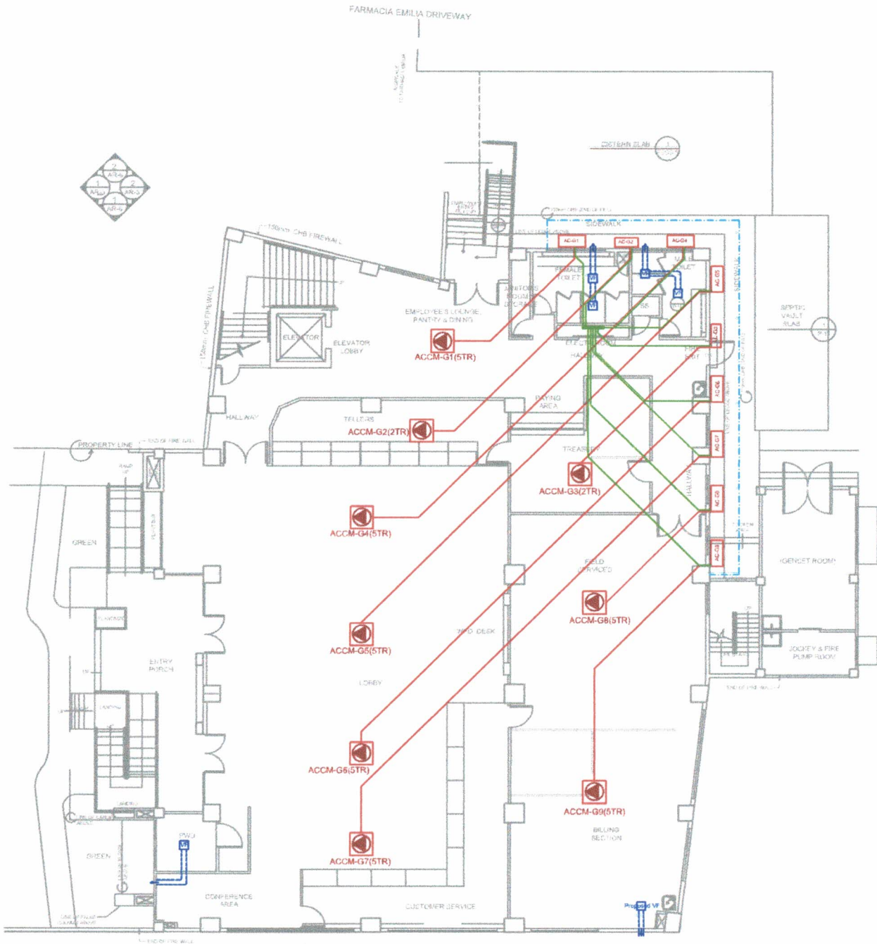
GROUND FLOOR AIRCON AND VENTILATION LAYOUT
