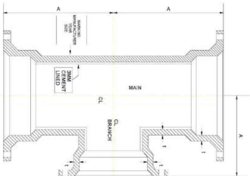
FULL SECTION VIEW OF CAST IRON MECHANICAL TEE
